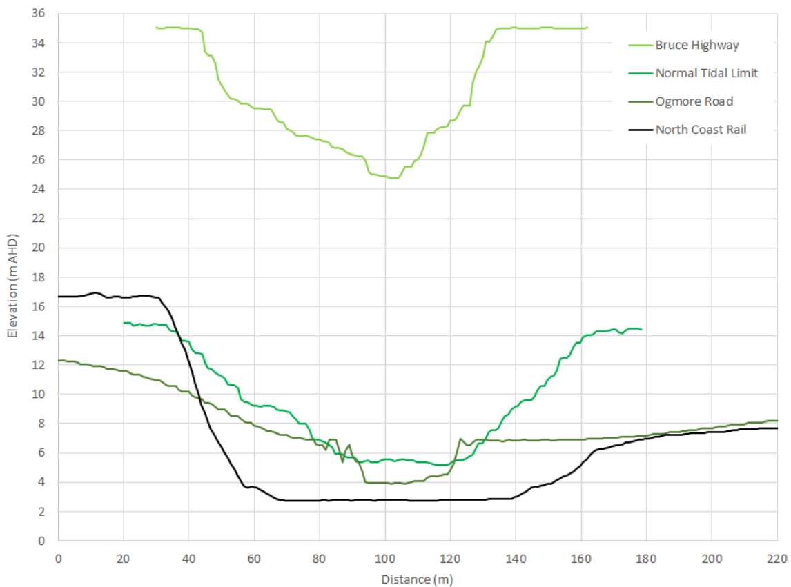
Figure 4-15 Storm tides at four locations
