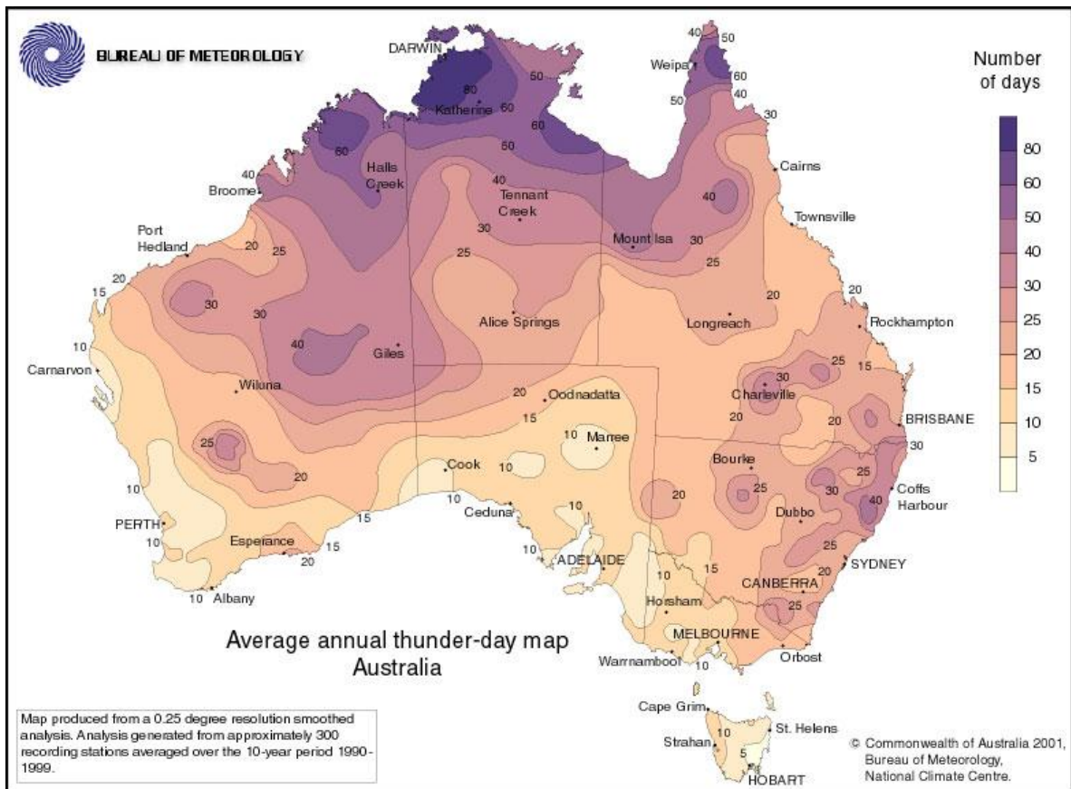
Figure 4-11 Average annual thunder-day map
