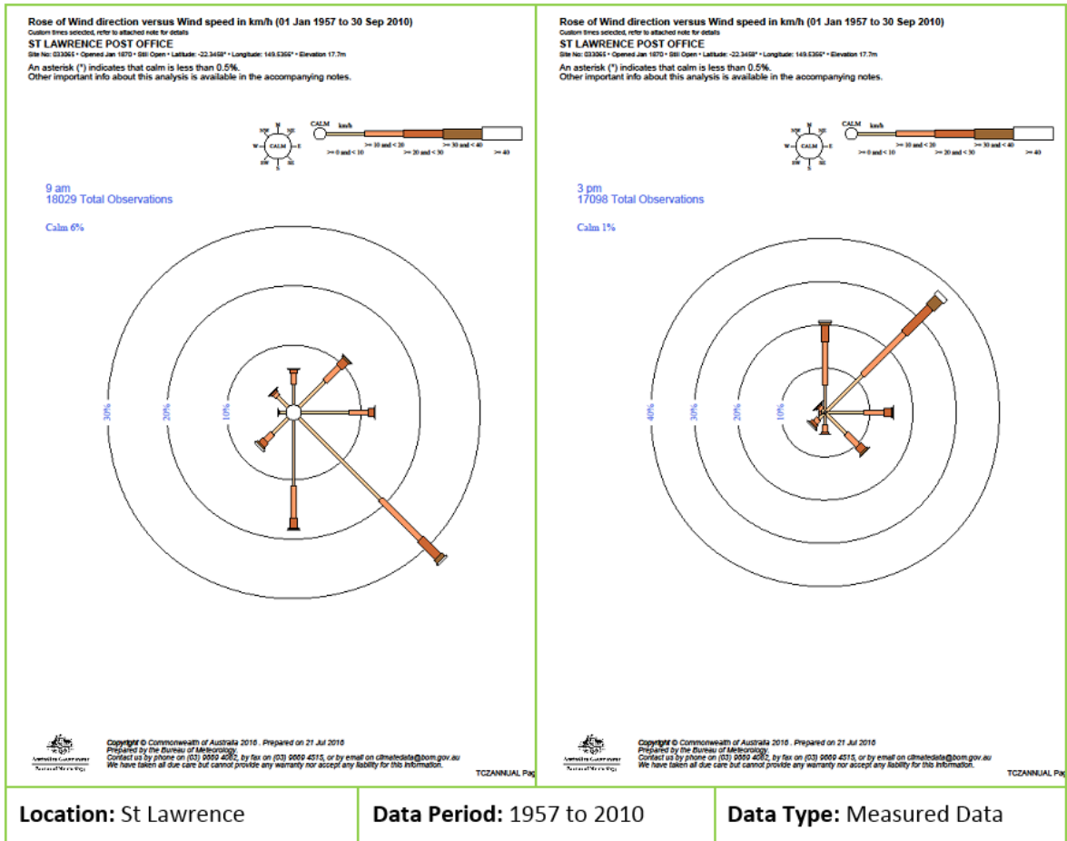
Figure 4-6 Annual wind rose
